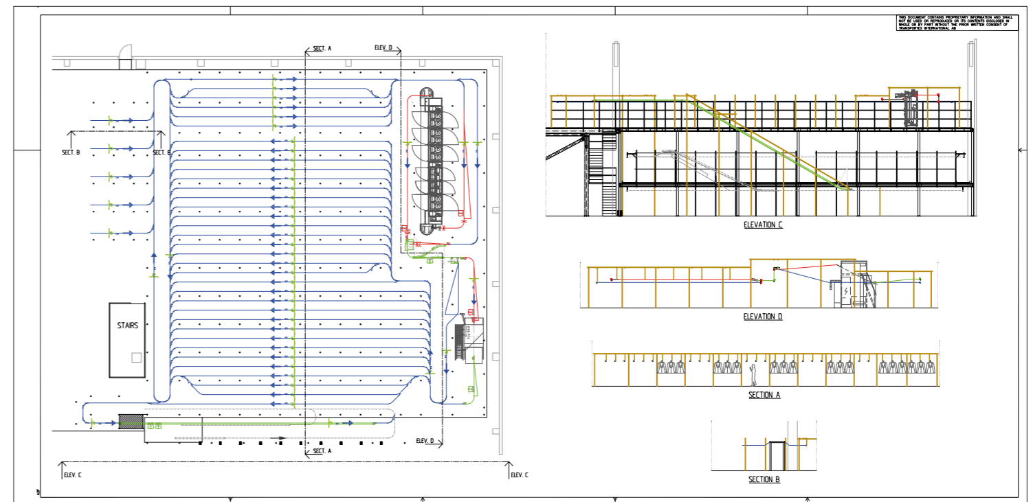
Automatic feeding into a bagging machine.
